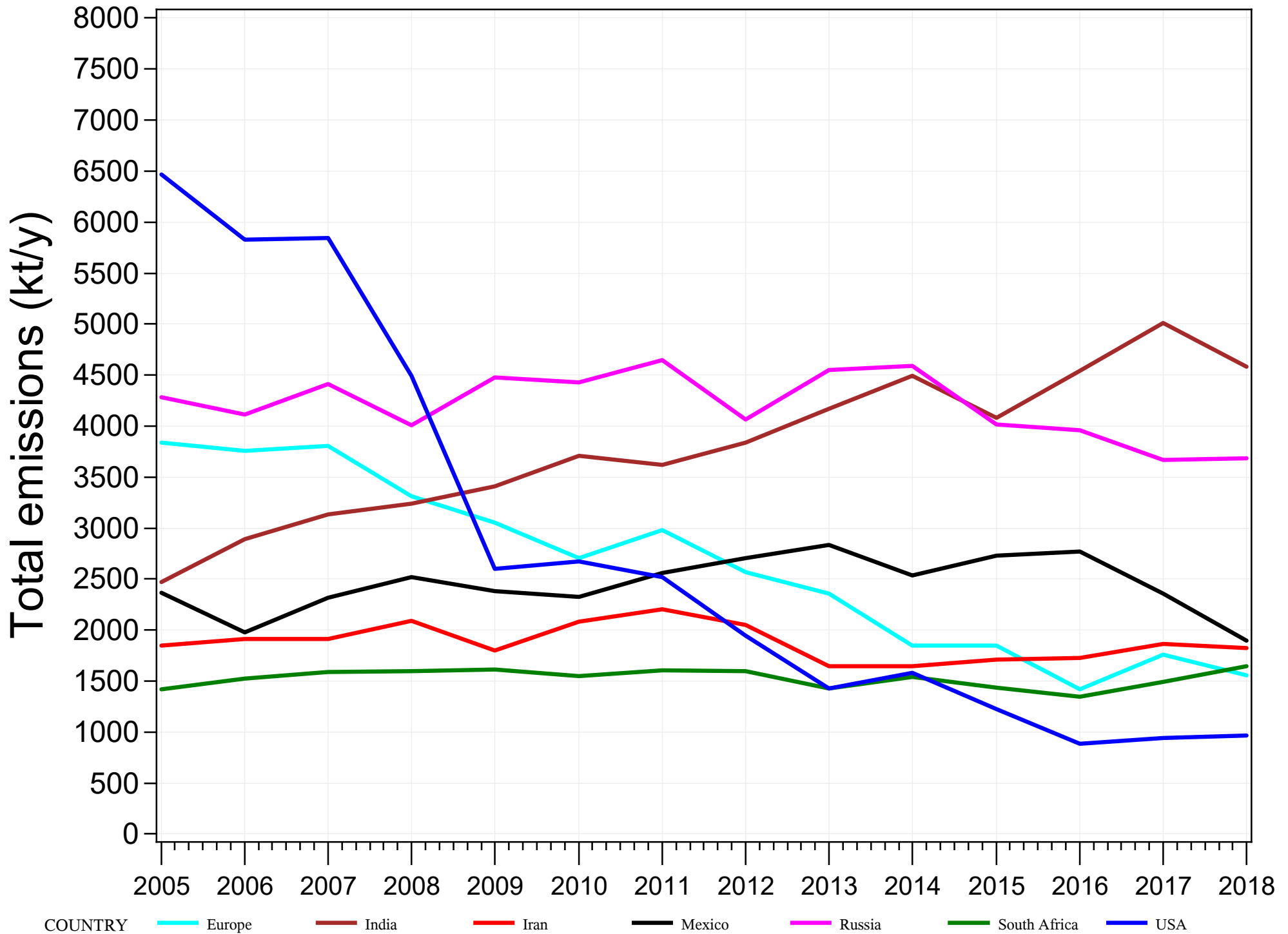
Total Annual Emissions by Country without China
