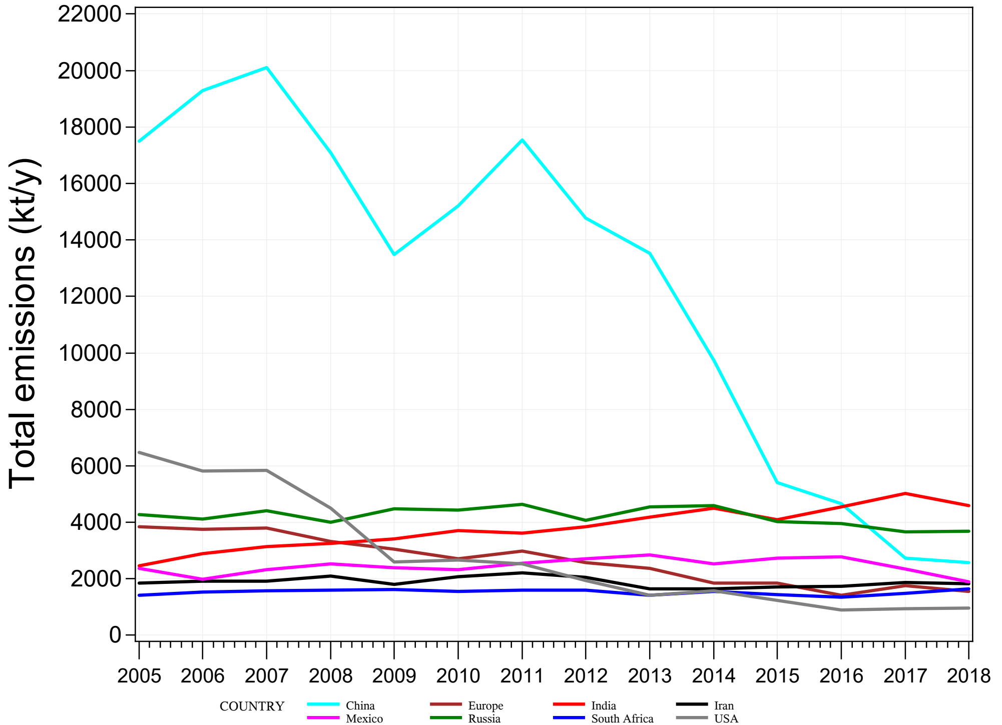
Total Annual Emissions by Country
