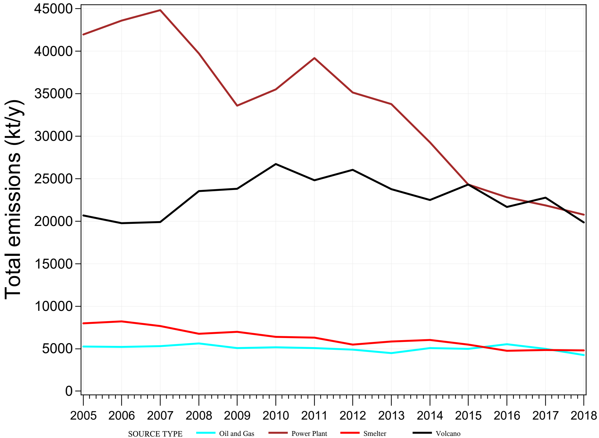
Total Annual Emissions by Source Type
