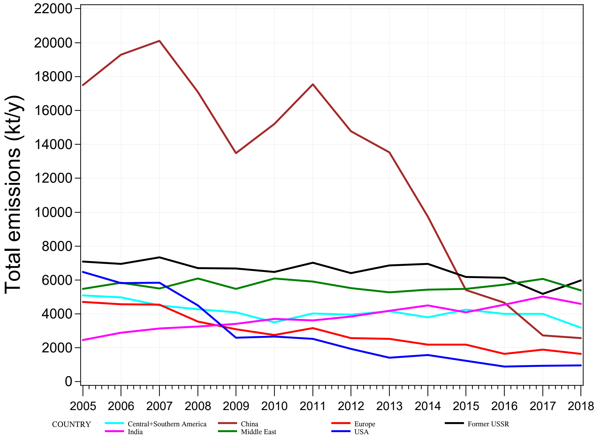
Total Annual Emissions by Region
